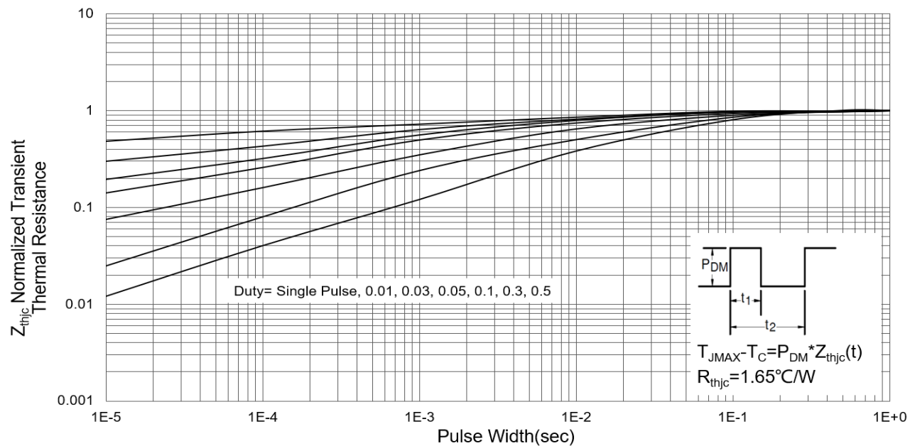
Fig11 Normalized Transient Impedance
