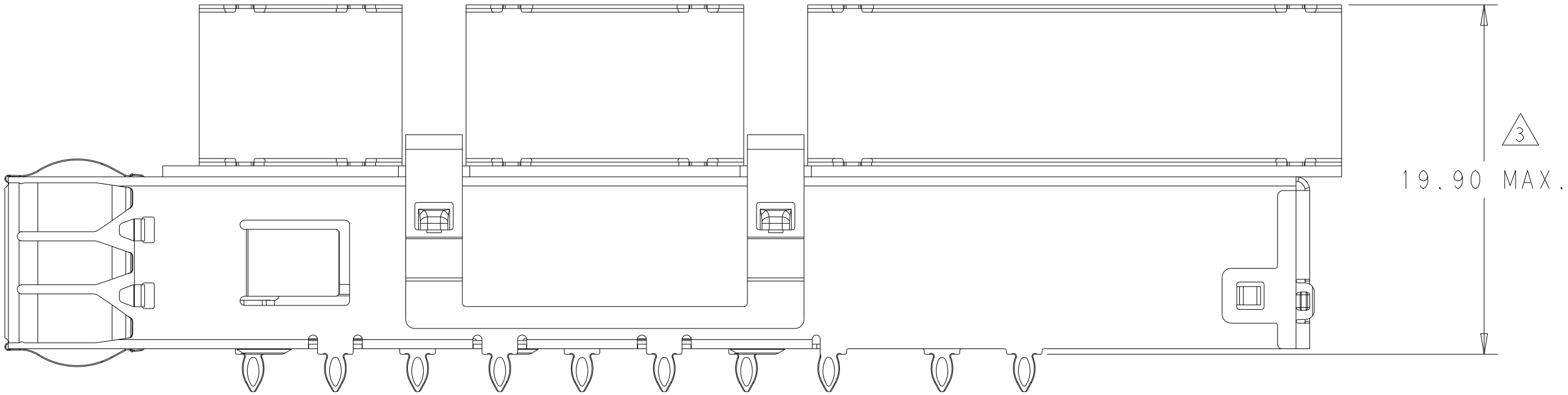
1-2361706-1 AS SHOWN SAME AS 2361706-1 EXCEPT WITHOUT REAR PIN SCALE 4:1
