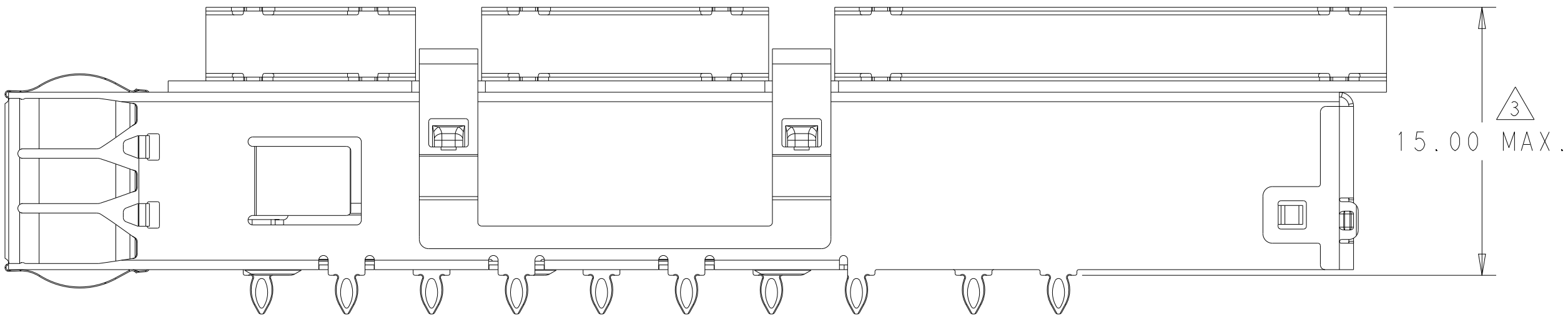
1-2361706-2 AS SHOWN SAME AS 2361706-2 EXCEPT WITHOUT REAR PIN SCALE 4:1
