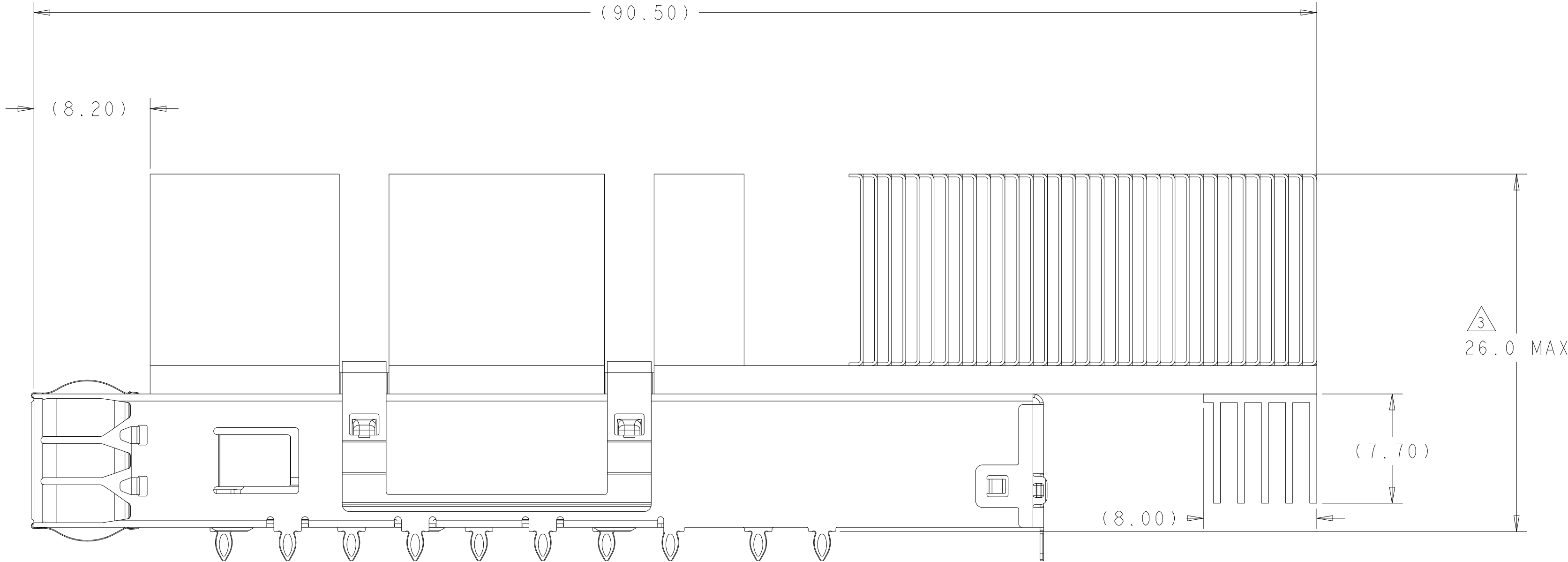
2-2361706-1 SAME AS -1 EXCEPT HS SCALE 4:1
