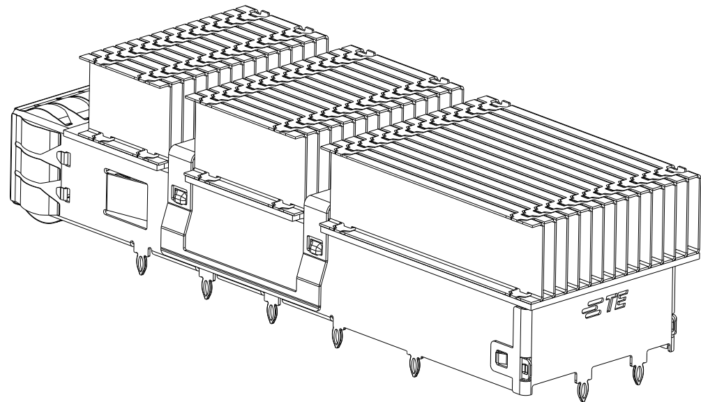
2361706-5 3D VIEW SCALE 2:1
