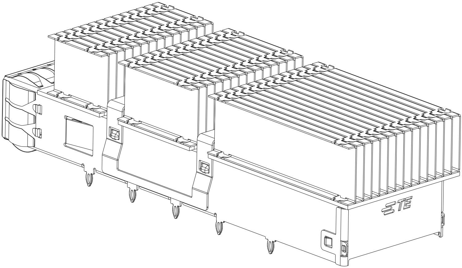
1-2361706-1 AS SHOWN SCALE 3:1
