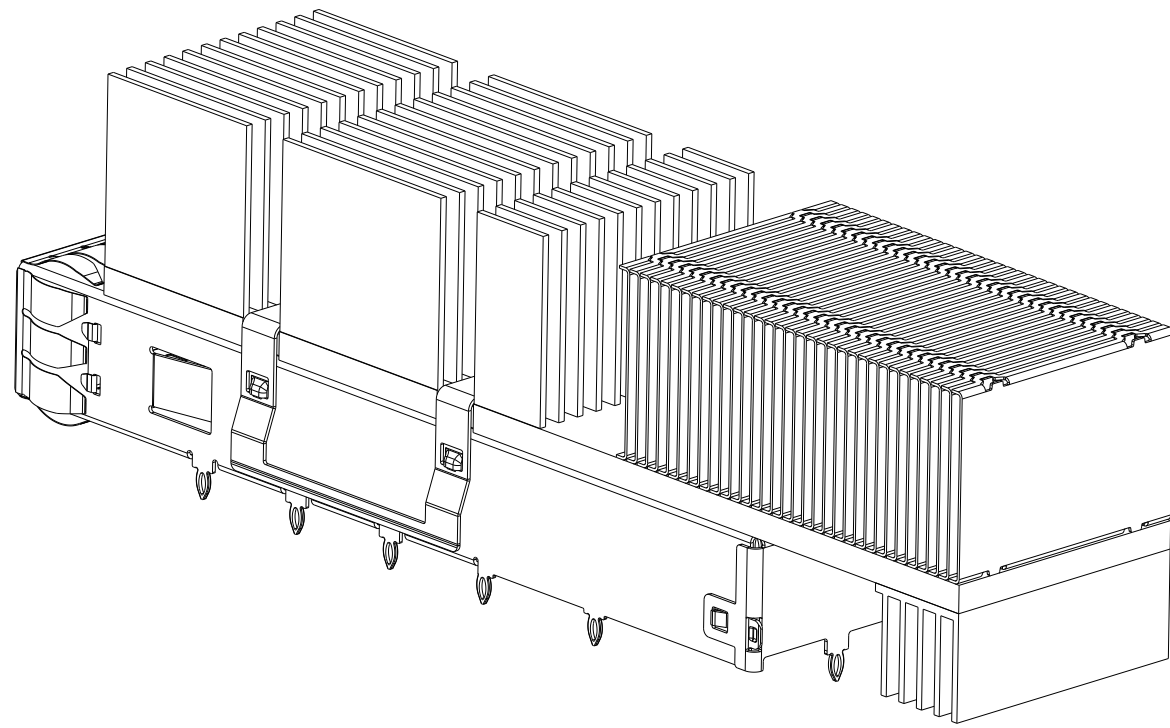
2-2361706-1 AS SHOWN SCALE 2:1
