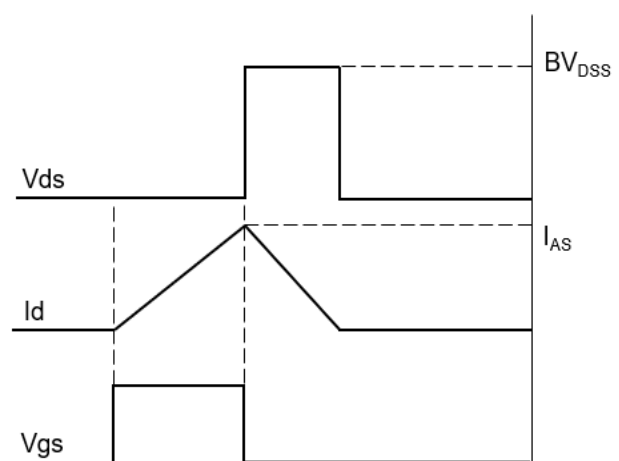
Fig11 EAS Waveform
