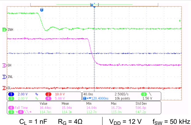
Figure 8-3. GH Fall Time and INH to GH Turn-off Propagation Delay
