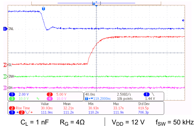
Figure 8-4. GL Rise Time and \overline{\text{INL}} to GL Turn-on Propagation Delay
