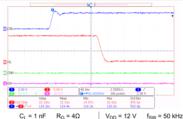
Figure 8-2. GL Fall Time and \overline{\text{INL}} to GL Turn-off Propagation Delay
