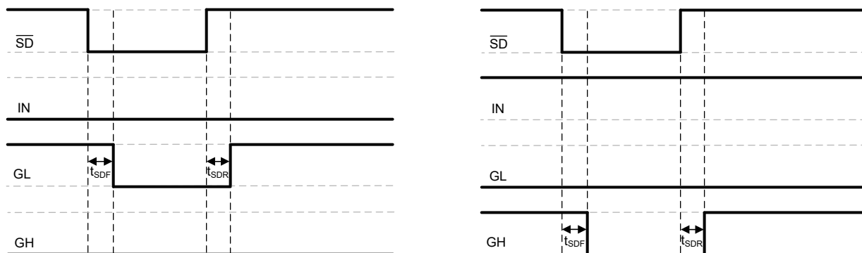
Figure 6-2. Shutdown Timing Diagram
