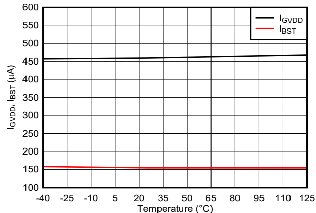
Figure 6-6. Quiescent Currents vs Temperature
