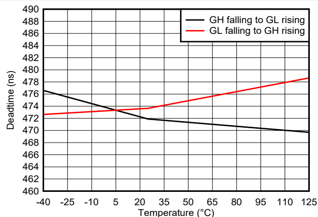
Figure 6-8. Deadtime vs Temperature
