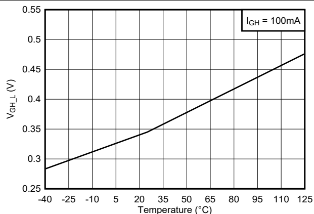
Figure 6-12. GH Output Low Voltage vs Temperature
