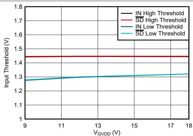
Figure 6-16. Input Voltage Thresholds vs Supply Voltage
