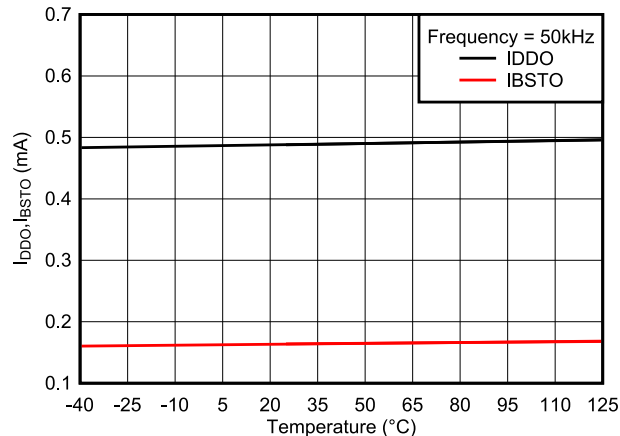
Figure 6-5. Operating Currents vs Temperature
