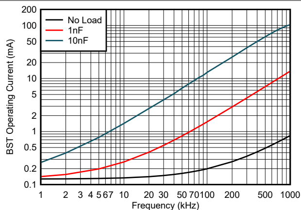
Figure 6-4. BST Operating Current vs Frequency
