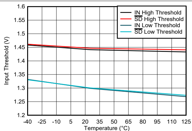
Figure 6-15. Input Voltage Thresholds vs Temperature
