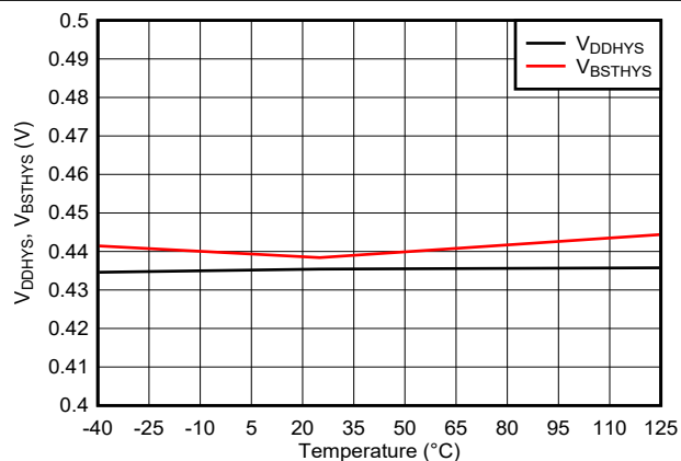
Figure 6-14. GVDD and BST UVLO Hysteresis vs Temperature
