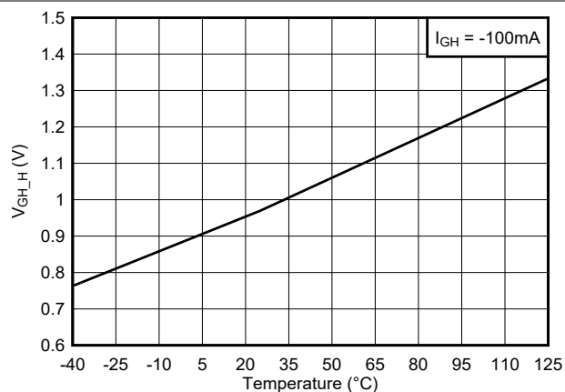
Figure 6-10. GH Output High Voltage vs Temperature
