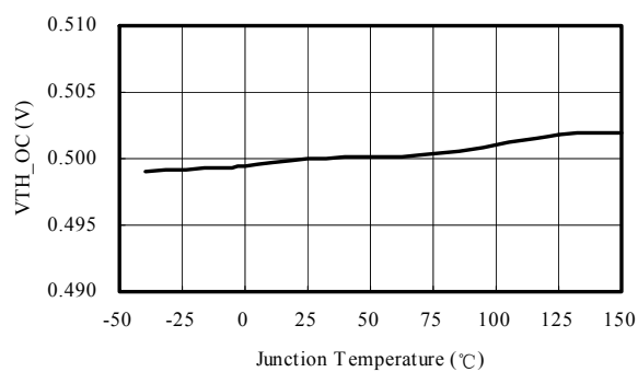
(f) V TH_OC vs Tj
