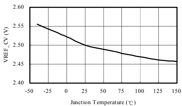
(e) V REF_CV vs Tj
