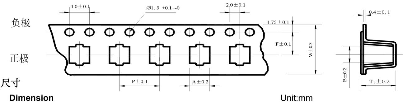
Drawing 1 (for Ø4 ~ Ø10) Unit:mm
