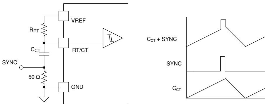
Figure 8-5. Oscillator Synchronization Circuit
