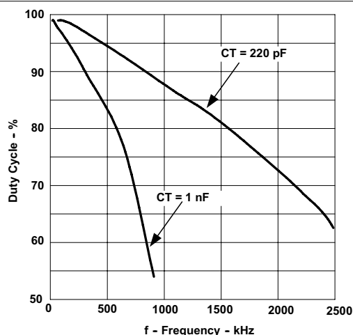
Figure 7-18. Maximum Duty Cycle vs Oscillator Frequency
