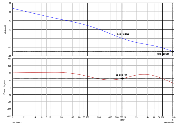
Figure 9-7. 40 V_{IN} , Maximum Load (1.33 A)
