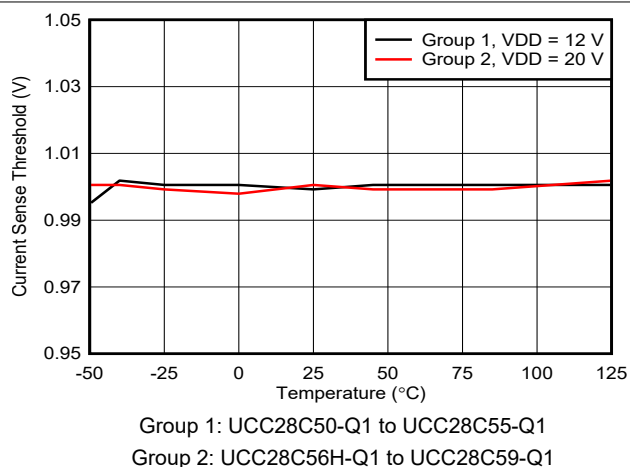
Figure 7-21. Current Sense Threshold Voltage vs Temperature
