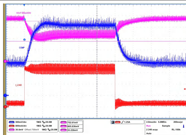
Figure 9-19. PWM Switching at 800 V IN , 40 W
