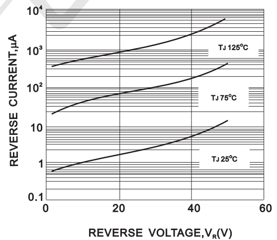
FIG. 2-TYPICAL REVERSE CHARACTERISTIC
