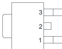
TO252-2
