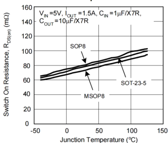
Switch On Resistance vs. Junction Temperature
