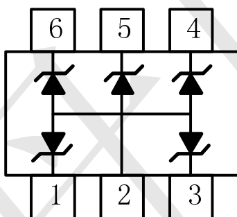
Pin Configuration
