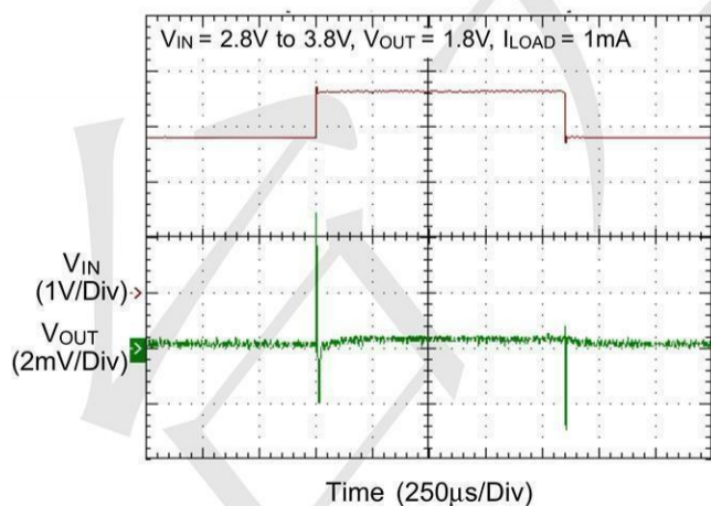
Line Transient
