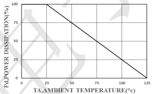
FIG 4. DERATING CURVE ( P_d - T_A )
