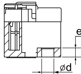
B-B (1:1)
