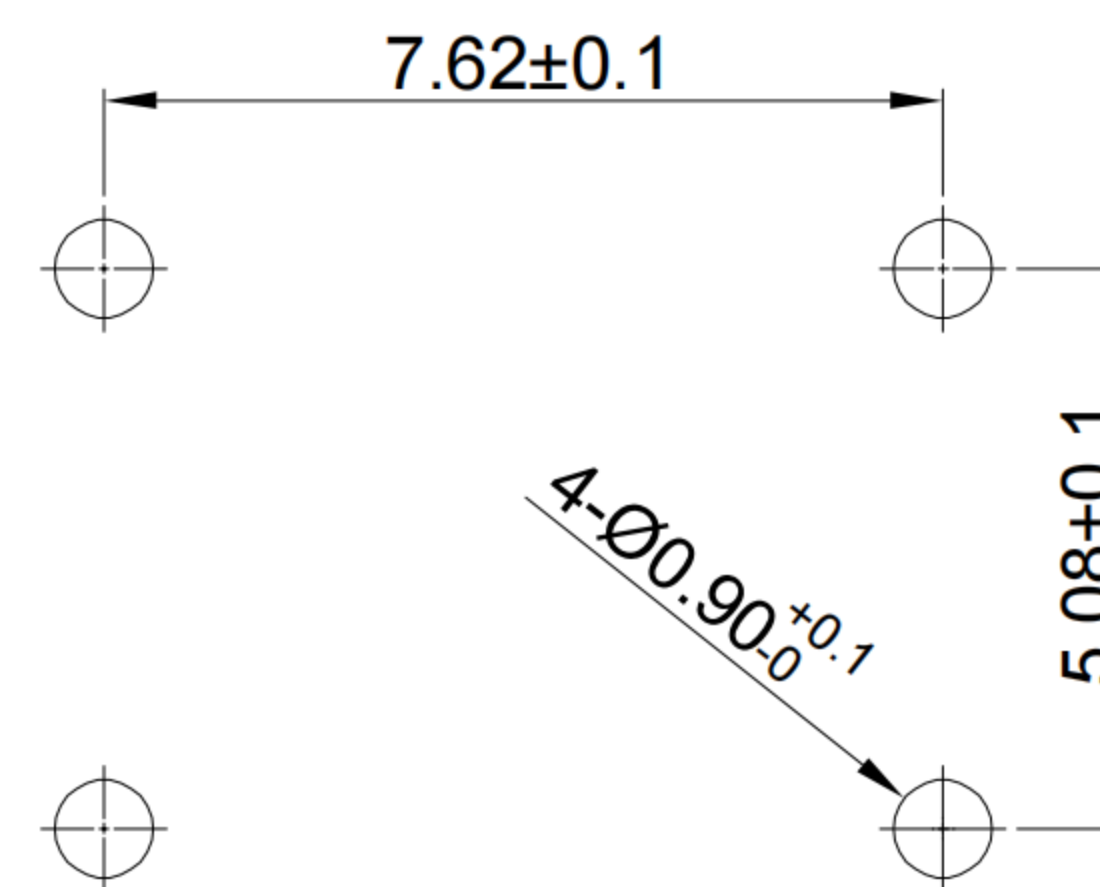
RECOMMENDED PCB LAYOUT TOLERANCE:±0.05
