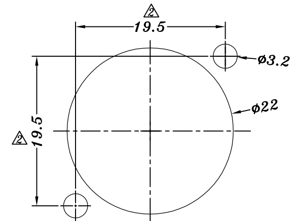
PANEL LAYOUT
