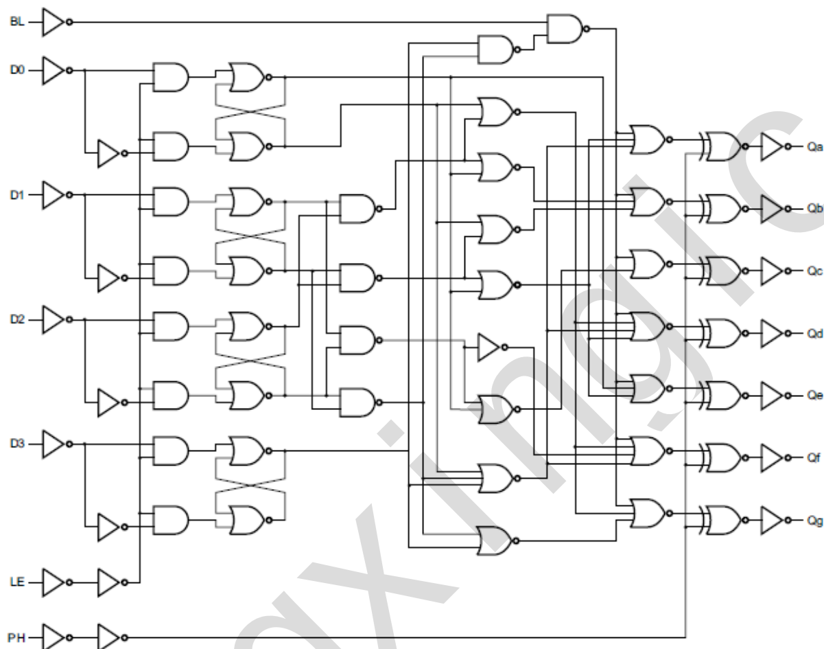
Figure 1. Functional diagram
