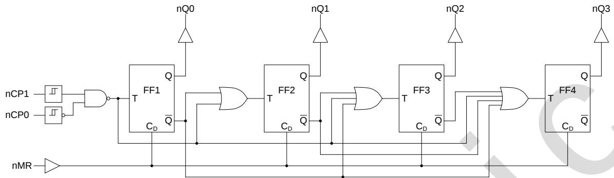
Figure 1. Functional diagram
