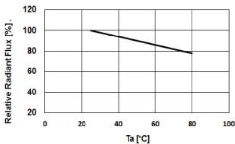
Fig.3 – Relative Radiant Flux (@500mA) vs. Ambient Temperature
