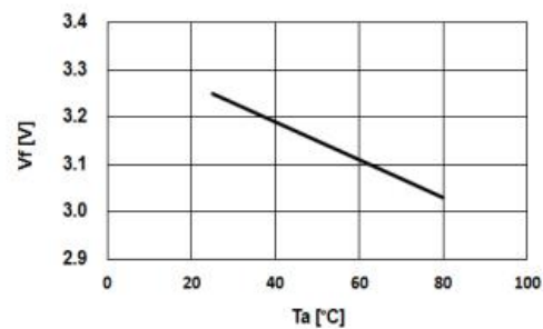
Fig.4 – Forward Voltage (@500mA) vs. Ambient Temperature
