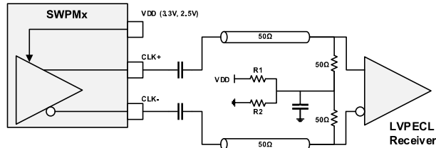
AC-Coupled Self-Biased LVEPCL - 50 Ω w/VTT Bias
