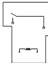
接线图(底视图) Installation hole bitmap (Bottom view)
