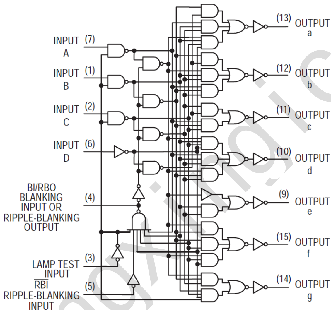
Figure 1. Logic diagram
