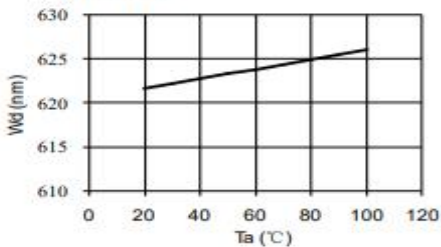
Fig.5-Dominant Wavelength (@150mA) vs. Ambient Temperature
