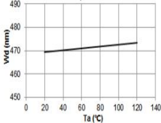
Fig.5-Dominant Wavelength (@120mA) vs. Ambient Temperature
