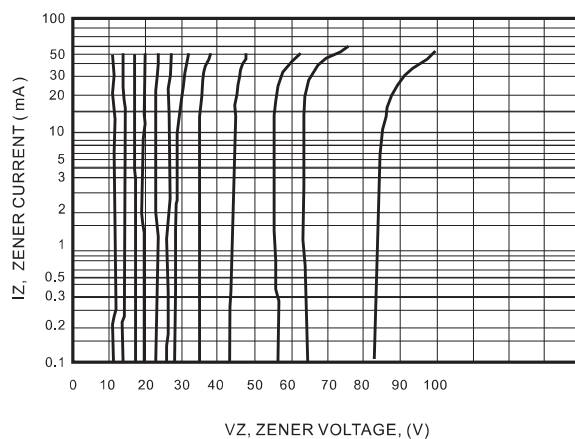
FIG.7 VZ = 12 Thru 82 Volts
