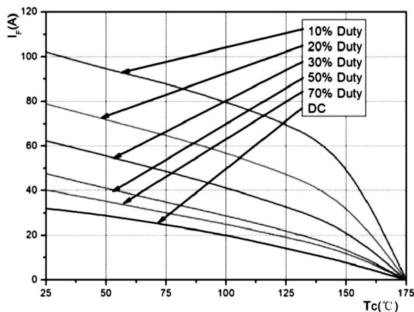
Figure 3. Load current
