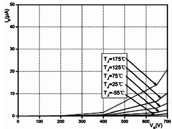
Figure 2. Reverse Characteristics
