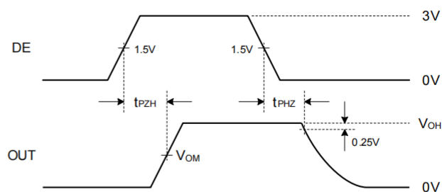
Fig. 5. Driver Enable and Disable Times, Output High
