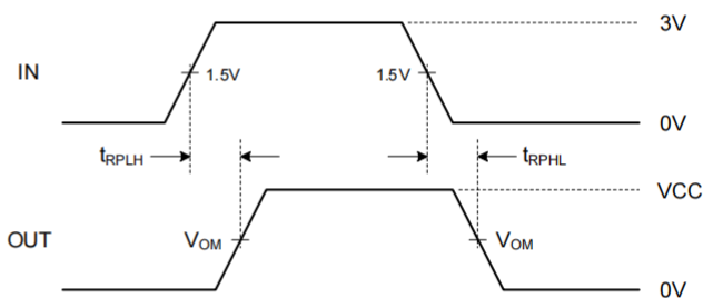
Fig. 7. Receiver Propagation Delay
