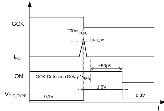
Figure 11: SCP Behavior
