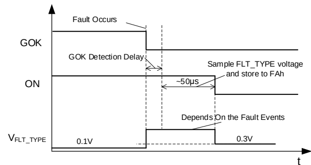
Figure 14: FLT_TYPE Indication
