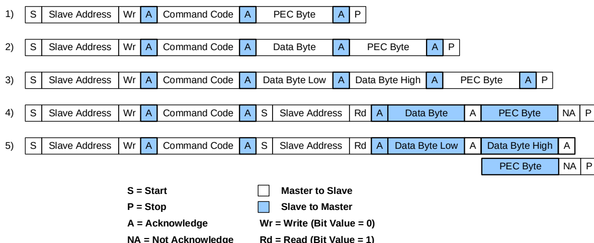
Figure 21: Supported PMBus/I²C Transmission Structure with PEC
