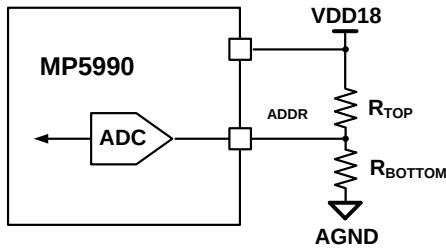
Figure 19: Recommended Circuit Design for PMBus Address Pin Set
