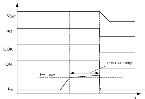
Figure 9: Total OCP Behavior
