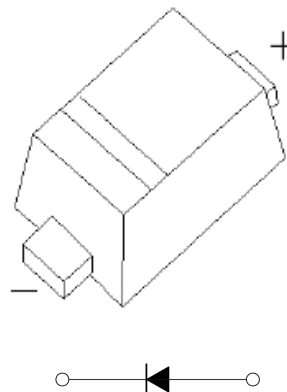
SOD-523
