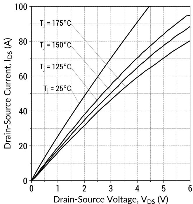
Figure 3: Output Characteristics ( V_{GS} = 20\text{ V} )
