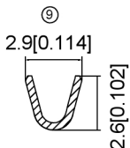
SECTION B-B SCALE 1:1
