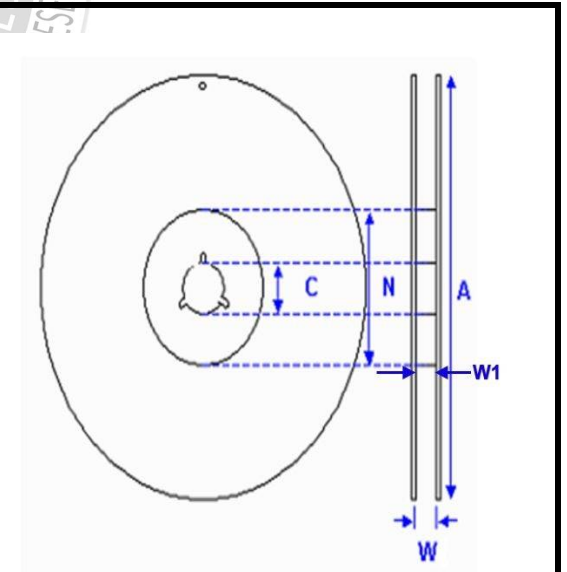
Fig. 9.3 The dimension of reel
