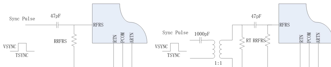
Figure 22 Synchronization
