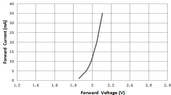
伏安特性曲线 Forward Current VS. Forward Voltage ( T_a=25^{\circ}\text{C} )
