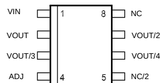
SOP-8
