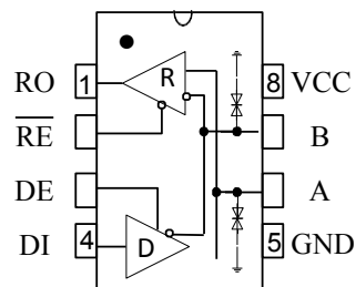
Figure 1 SP3485EEN-EV pin configuration
