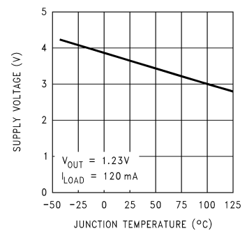
Supply Voltage
