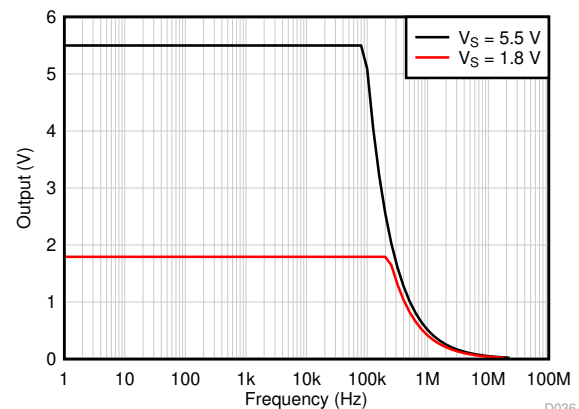
Figure 6-50. Maximum Output Voltage vs Frequency
