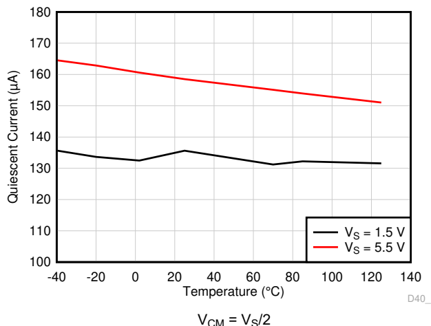
Figure 6-37. Quiescent Current vs Temperature
