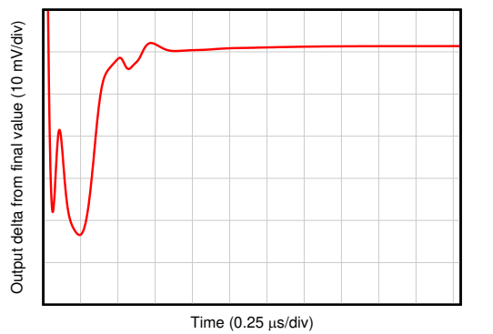
Figure 6-45. Small-Signal Step Response
