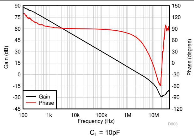
Figure 6-18. Open-Loop Gain and Phase vs Frequency
