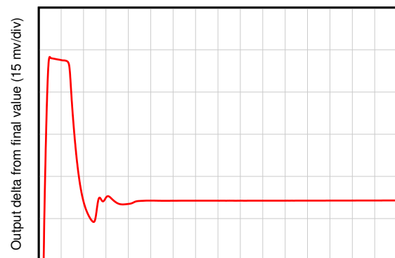
Figure 6-46. Large-Signal Step Response
