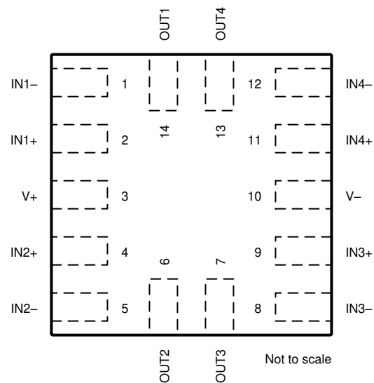
Figure 5-11. OPA4310 RUC Package, 14-Pin X2QFN (Top View)
