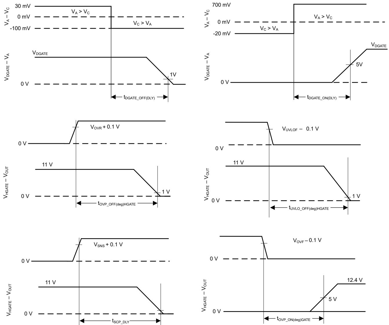
Figure 8-1. Timing Waveforms
