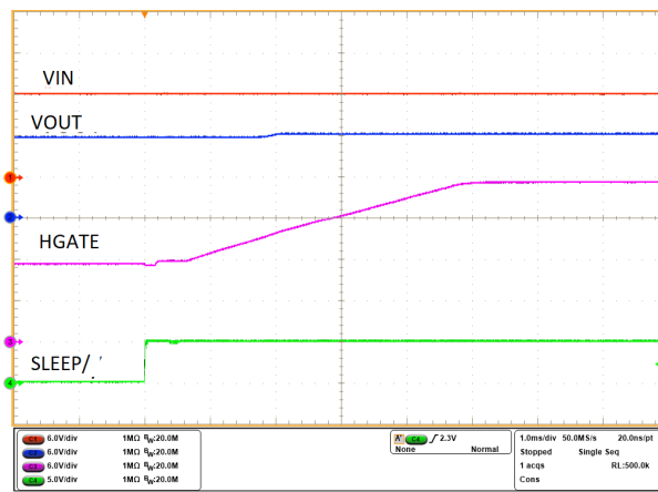
Figure 10-21. SLEEP Mode Exit (SLEEP = High, EN = High)
