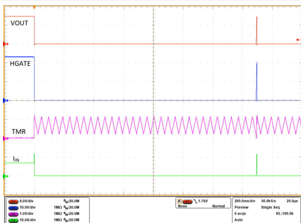
Figure 10-13. Output Overcurrent Protection (TIMER Duration 1 ms): Auto Retry
