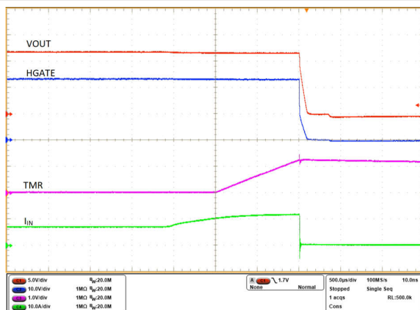
Figure 10-12. Output Overcurrent Protection (TIMER Duration 1 ms)
