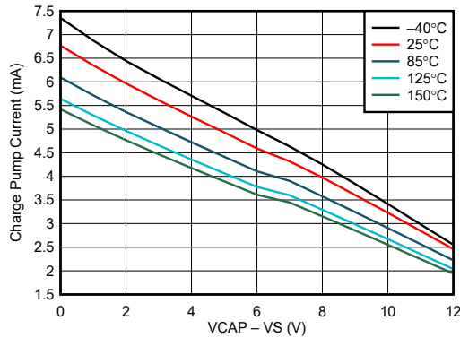
Figure 7-7. Charge Pump V-I Characteristics at V_S \geq 12 V (LM74910-Q1)
