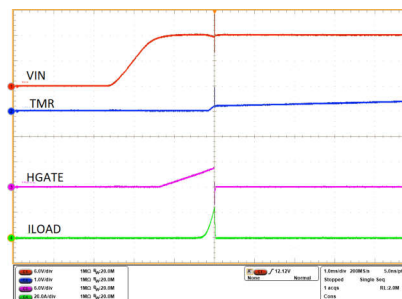
Device Start-Up With Overcurrent Protection
