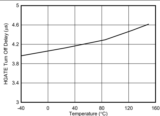
Figure 7-20. HGATE Turn Off Delay During OV
