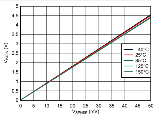
Figure 7-22. Current Monitor Output vs Sense Voltage ( R_{MON} = 5k\Omega , R_{SET} = 50\Omega )
