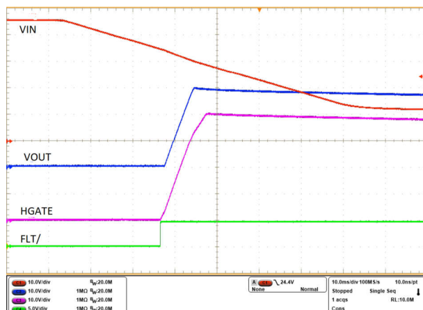
Figure 10-15. Overtoltage Recovery
