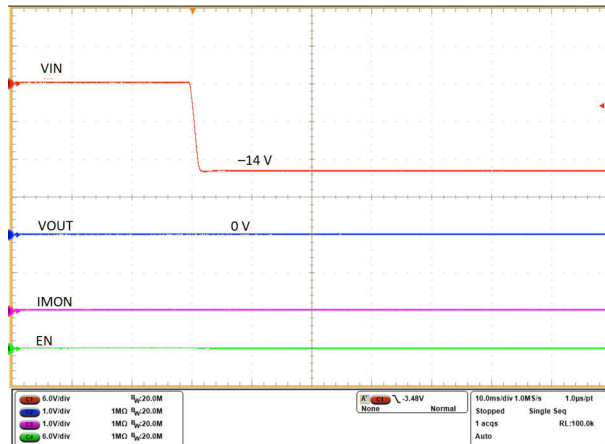
Figure 10-8. Reverse Input Voltage -14 V
