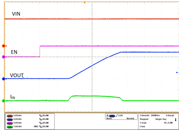
Figure 10-9. Inrush Current With No Load at Output
