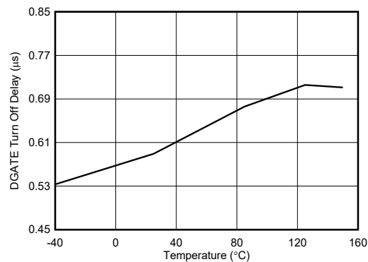
Figure 7-18. DGATE Turn OFF Delay
