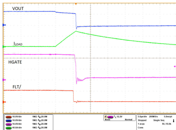
Figure 10-10. Output Short Circuit Protection (On-The-Fly)
