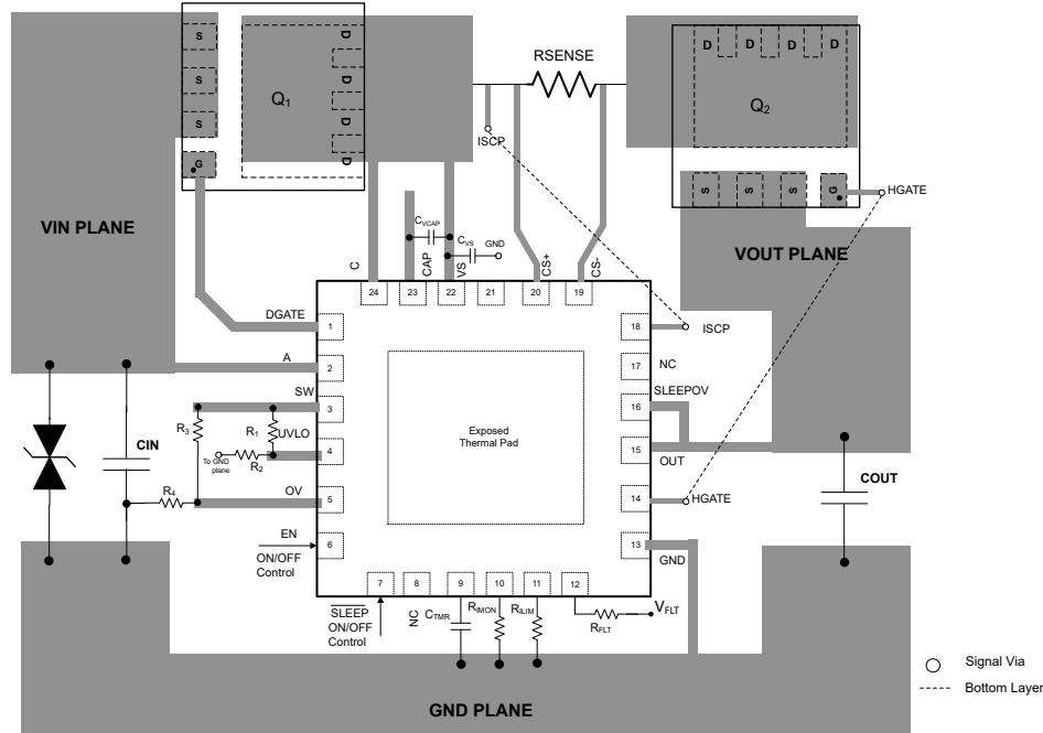
Figure 10-24. Example Layout
