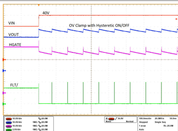
Figure 10-16. Overtoltage Clamp Response (OV Resistor Ladder Referred to VOUT)
