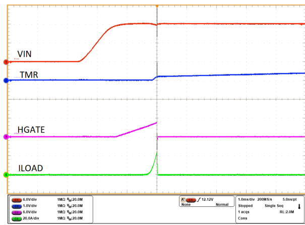
Figure 10-11. Device Start-Up With Output Short Circuit (TIMER Duration 1 ms)
