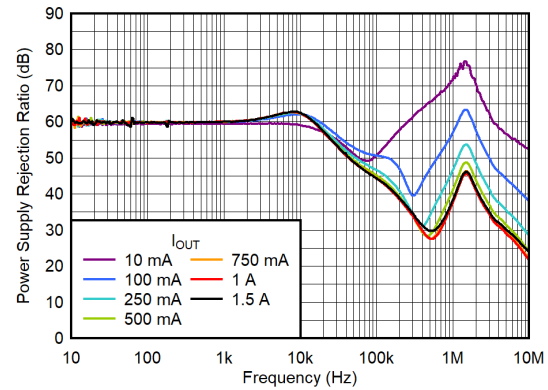
Figure 6-8. BIAS PSRR vs Frequency and I_{OUT}
