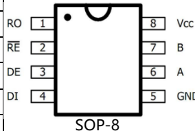
SOP-8
