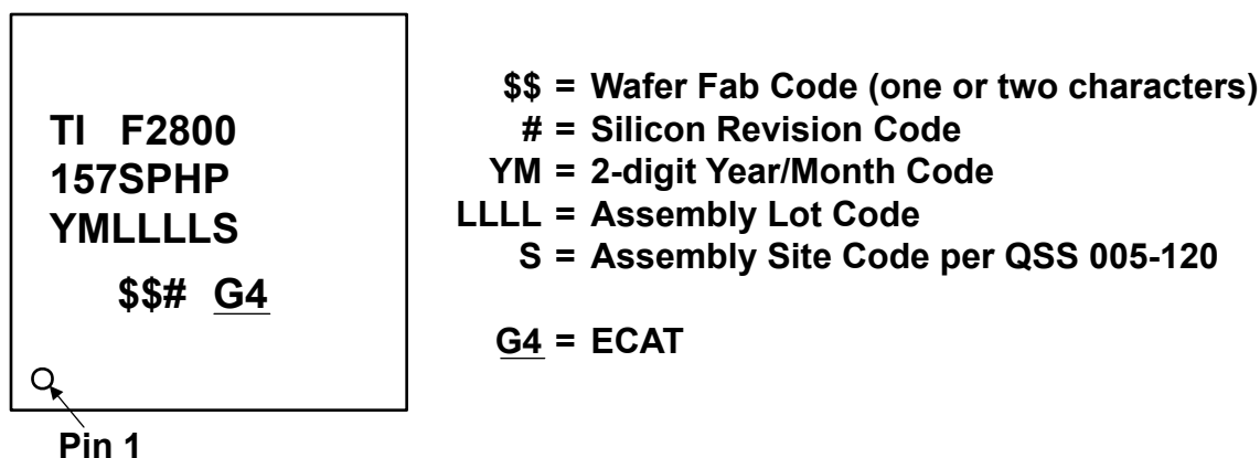
Figure 9-6. Package Symbolization for PHP Package
