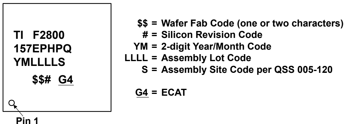
Figure 9-8. Package Symbolization for PHP Package (AEC-Q100 Grade 0 Qualification)
