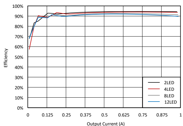
Figure 7-12. Efficiency at 13-V Input Voltage, 1-A Output Current
