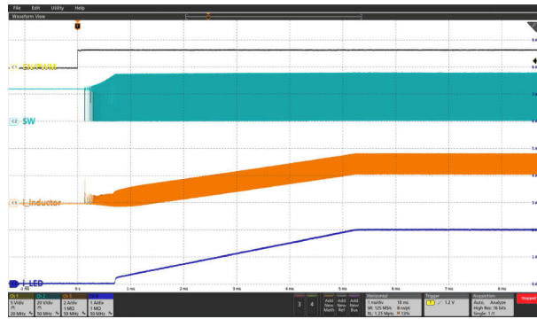
Figure 9-19. Start-Up at PWM PWM = 100%, 20 kHz
