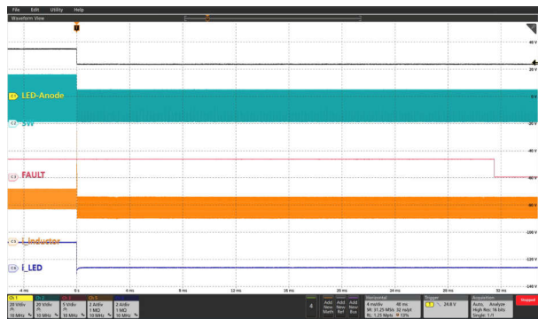
Black: PWM_{PWM} , Light Blue: SW, Red: FAULT, Orange: Inductor Current, Deep Blue: LED Current
