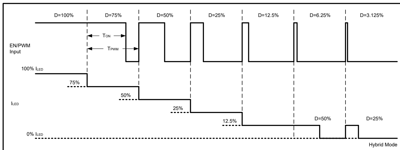
Figure 8-3. Hybrid Dimming
