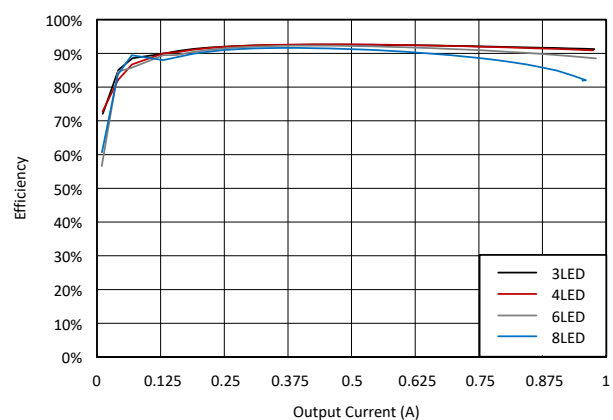
Figure 7-11. Efficiency at 7-V Input Voltage, 1-A Output Current
