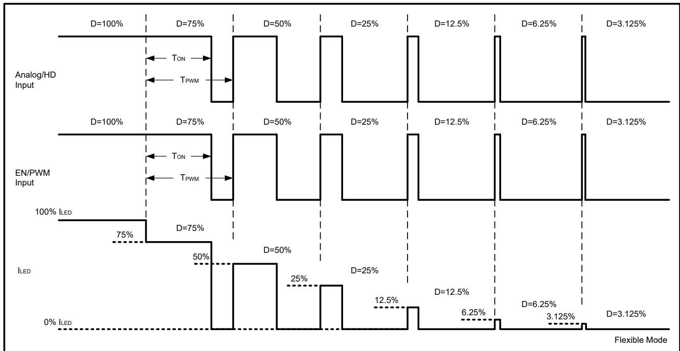
Figure 8-4. Flexible Dimming
