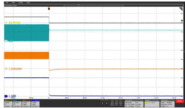
Figure 9-20. Shutdown at PWM PWM = 100%, 20 kHz
