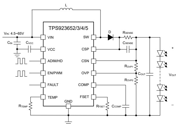
Simplified Schematic
