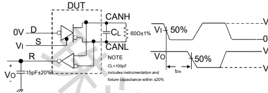
F7. tEN Test Circuit and Voltage Waveforms
