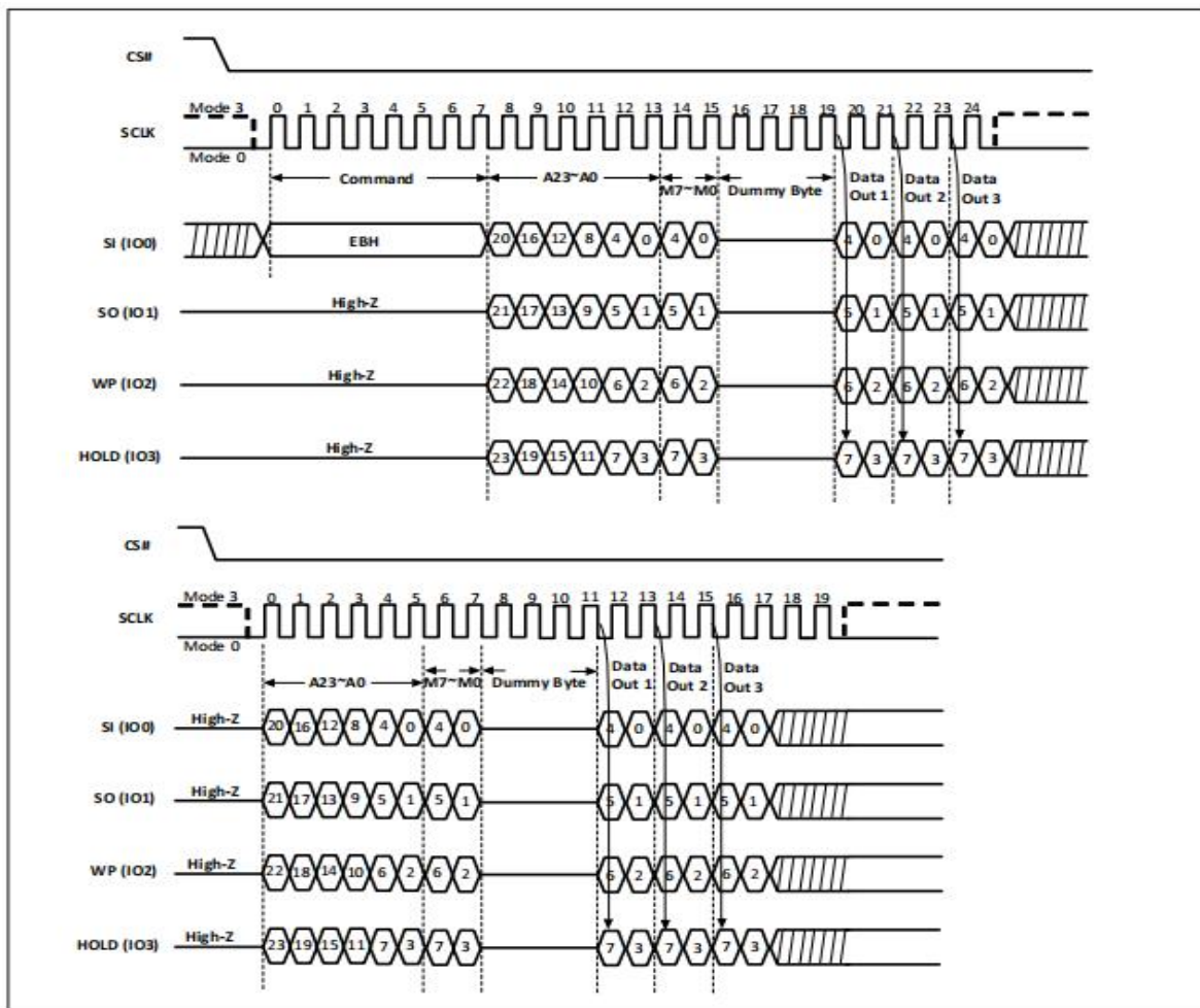
Figure-17. Quad I/O Fast Read with “Continuous Read Mode” Sequence Diagram (M5-4 = (1,0))
