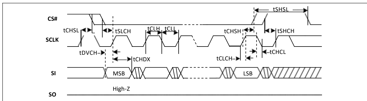
Figure-45. Serial Input Timing
