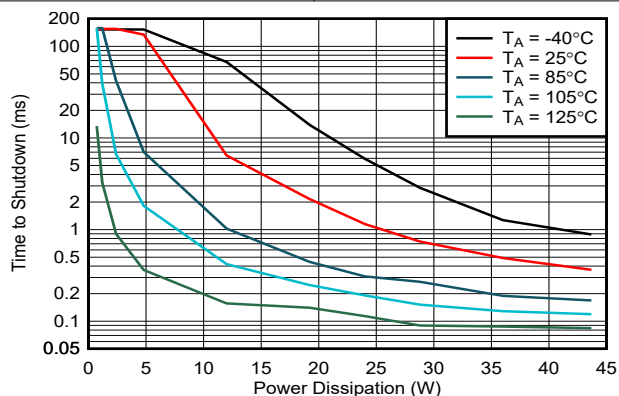
Figure 7-15. Thermal Shutdown Time vs Power Dissipation with V_{IN} = 24 V
