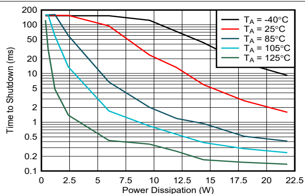
Figure 7-14. Thermal Shutdown Time vs Power Dissipation with V_{IN} = 12 V
