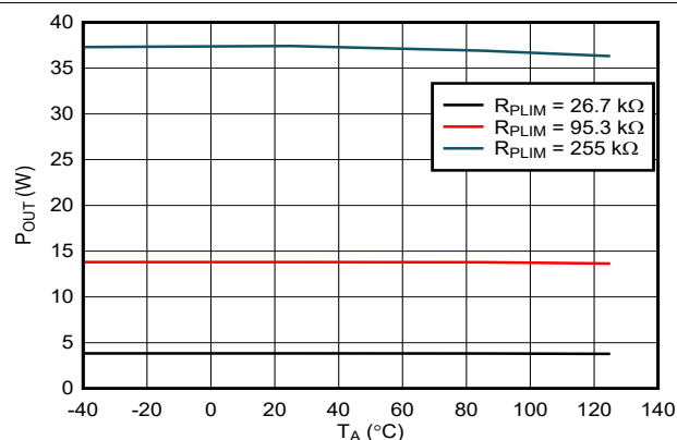
Figure 7-13. Output Power Limit vs Temperature for TPS16410 and TPS16411 with V_{IN} = 24 V
