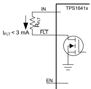
Figure 8-16. \overline{FLT} Output in the TPS1641x
