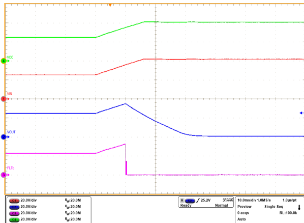
Figure 9-2. Overtoltage Protection up to 40 V
