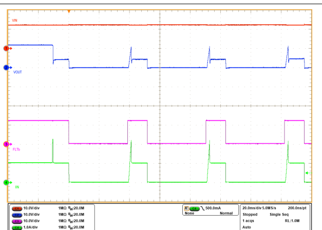
Figure 8-11. I_{OCP} \leq I_{OUT} < I_{fast-trip}
