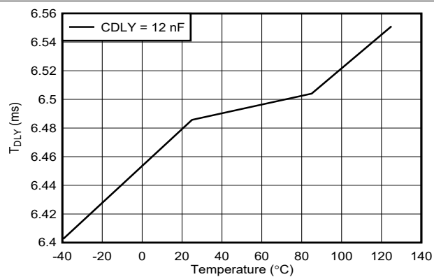
Figure 7-12. TDLY vs Temperature
