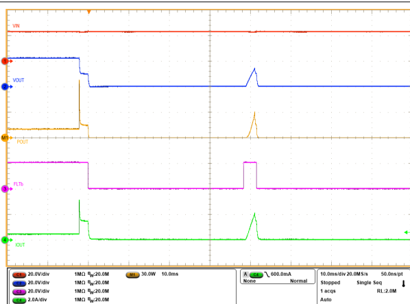
Figure 9-6. 15-W Power Limiting with TPS16410 ( I_{ocp} \leq I_{OUT} < I_{fast-trip} )
