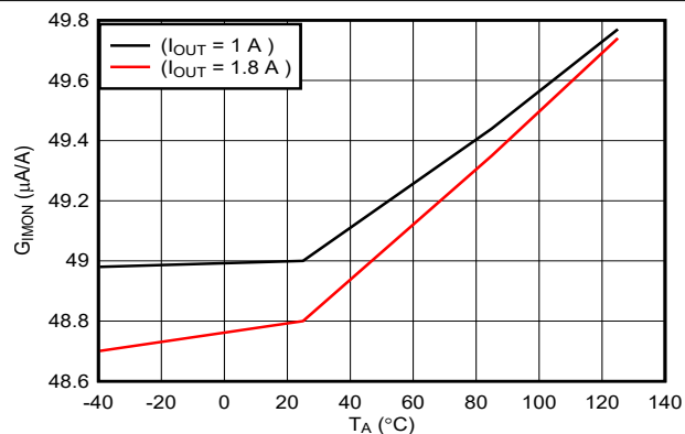
Figure 7-8. G IMON vs Temperature
