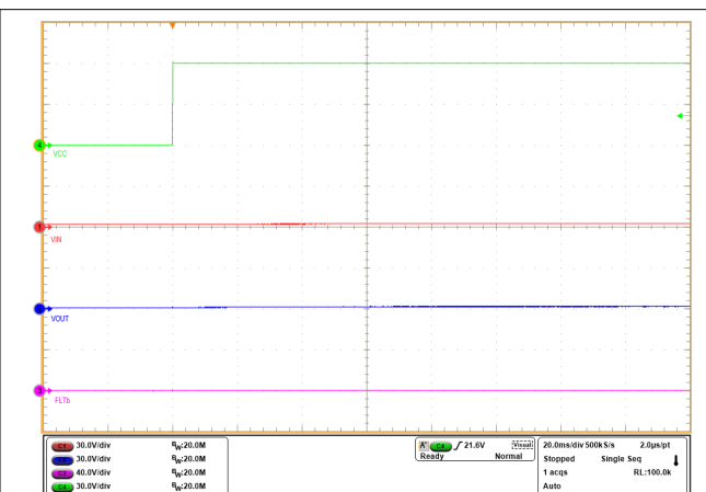
Figure 8-7. Hot Plug with External PFET for 60-V Input
