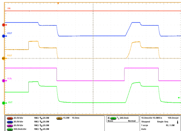
Figure 9-5. 15-W Power Limiting with TPS16410 ( I_{OUT} < I_{ocp} )
