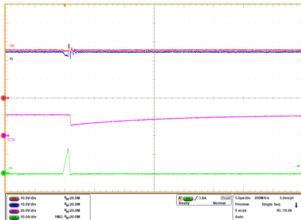
Figure 9-4. Output Short-Circuit Protection
