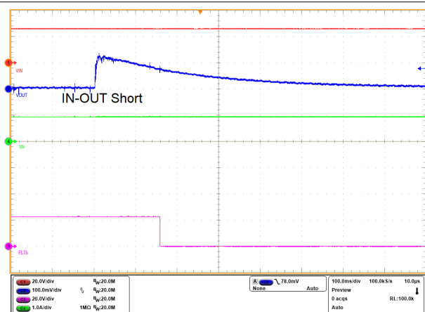
Figure 9-7. IN to OUT Short Detection with V_{IN} = 24 V
