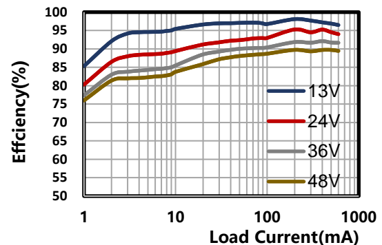
Efficiency (%) VOUT=12V
