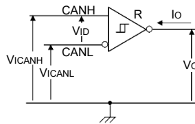
F5. Receiver Voltage and Current Definitions
