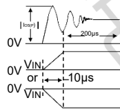
F9. Driver Short Circuit Current Test Circuit and Waveforms
