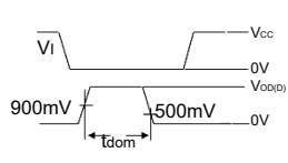
F10. Revealed Timeout Test Circuit and Waveforms
