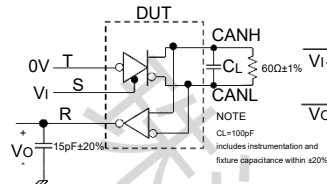
F7. tEN Test Circuit and Voltage Waveforms
