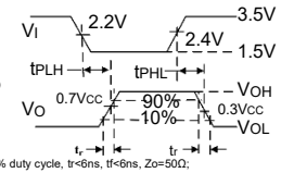
F6. Receiver test circuit and voltage waveform
