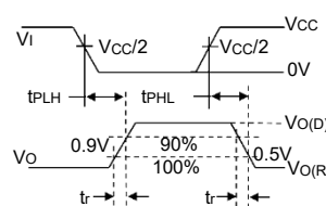
F4. Driver Test Circuit and Voltage Waveforms
