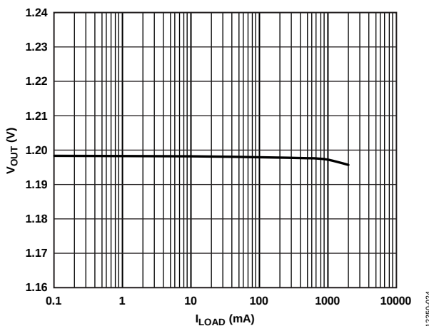
Figure 24. Output Voltage ( V_{OUT} ) vs. Load Current ( I_{LOAD} ), Adjustable Version, V_{OUT} = 1.2\text{ V}
