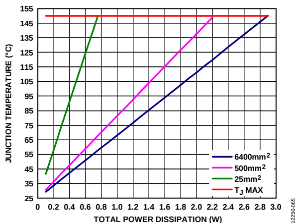
Figure 64. LFCSP, T_A = 25^\circ\text{C}
