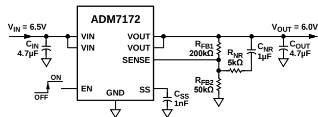
Figure 63. Noise Reduction Modification
