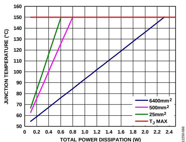
Figure 65. LFCSP, T_A = 50^\circ\text{C}
