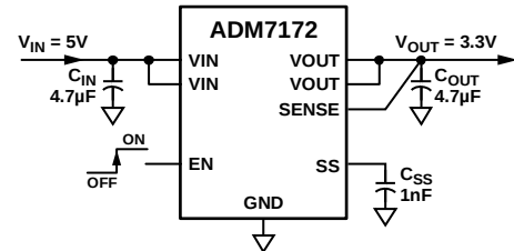
Figure 1. ADM7172 with Fixed Output Voltage, 3.3 V
