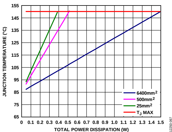
Figure 66. LFCSP, T_A = 85^\circ\text{C}
